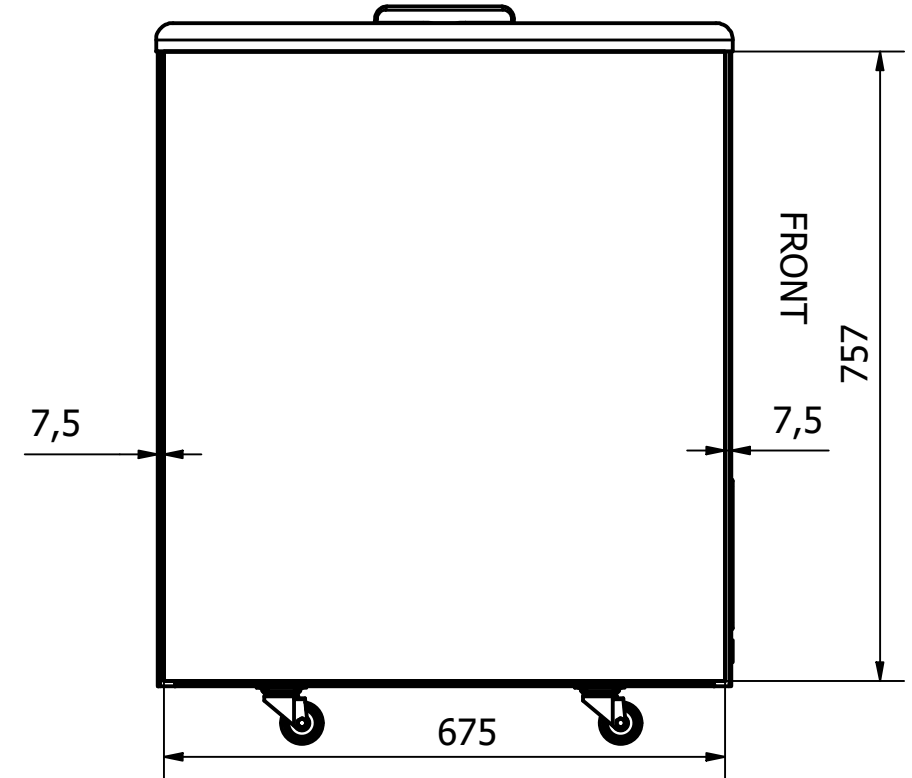
LEFT SIDE: Sticker 675 x 757 mm
