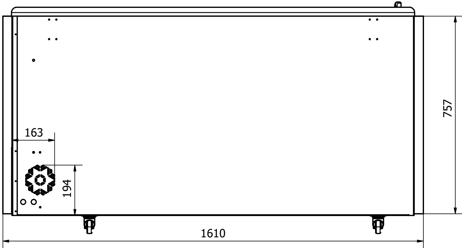
BACK: Sticker 1610 x 757 mm
